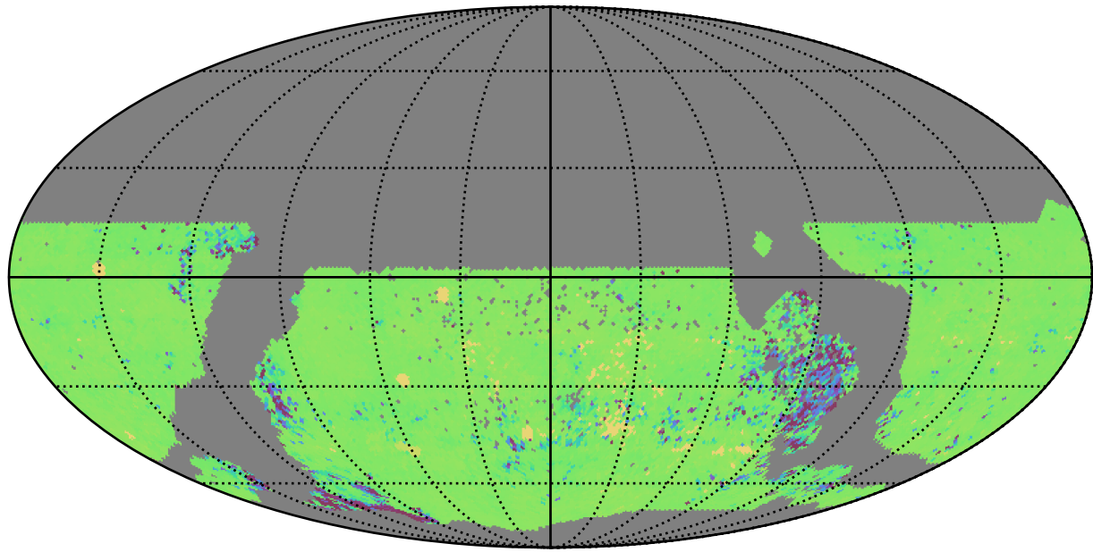
ddf_acor_sf15_lsf30_lsr10_v3.4_10yrs WFD ug bands: 75th Percentile Intranight Timespan
