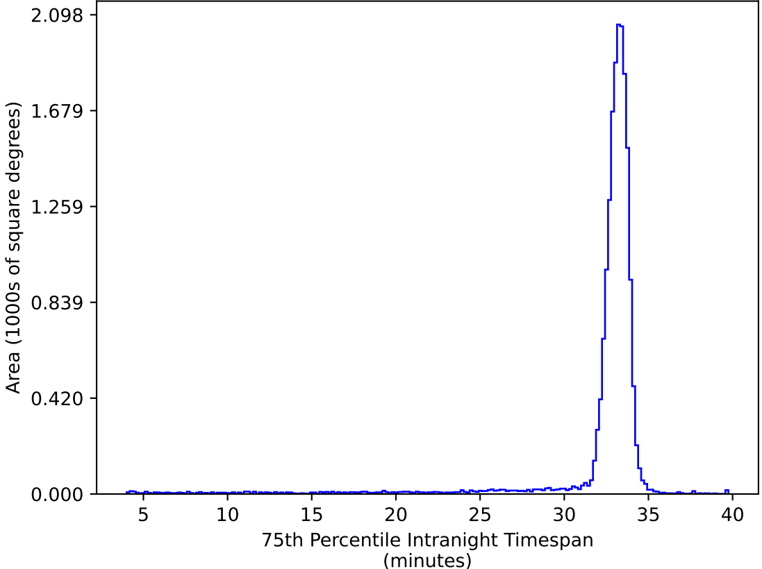
ddf_acor_sf15_lsf30_lsr10_v3.4_10yrs WFD ug bands: 75th Percentile Intranight Timespan
