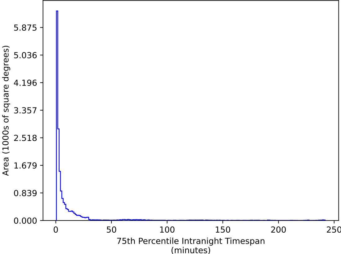
ddf_acor_sf15_lsf30_lsr10_v3.4_10yrs WFD u band: 75th Percentile Intranight Timespan
