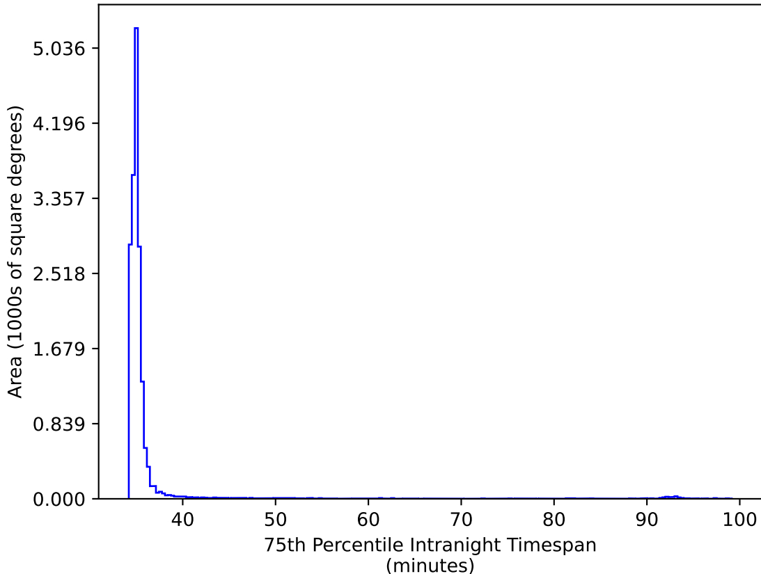
ddf_acor_sf15_lsf30_lsr10_v3.4_10yrs WFD ri bands: 75th Percentile Intranight Timespan
