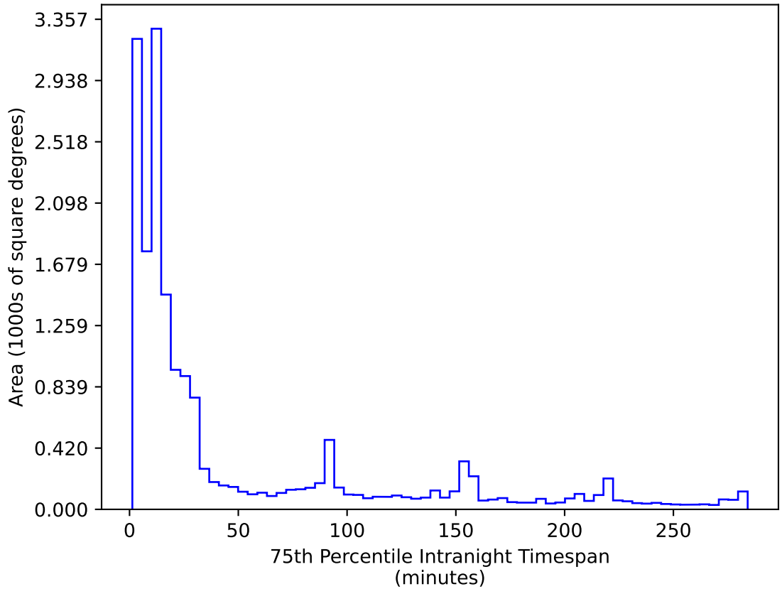
ddf_acor_sf15_ls30_lsr10_v3.4_10yrs WFD r band: 75th Percentile Intranight Timespan
