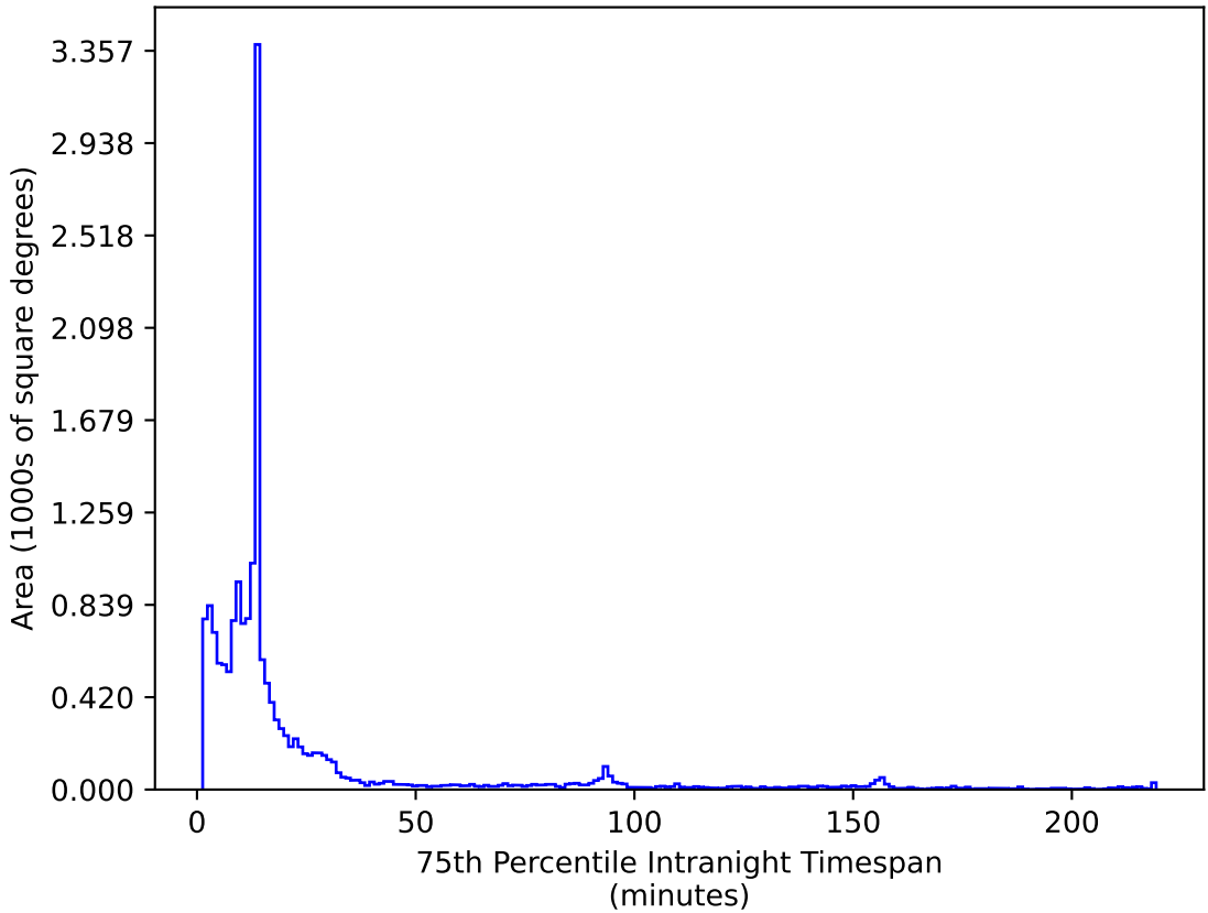
ddf_acor_sf15_lsf30_lsr10_v3.4_10yrs WFD i band: 75th Percentile Intranight Timespan
