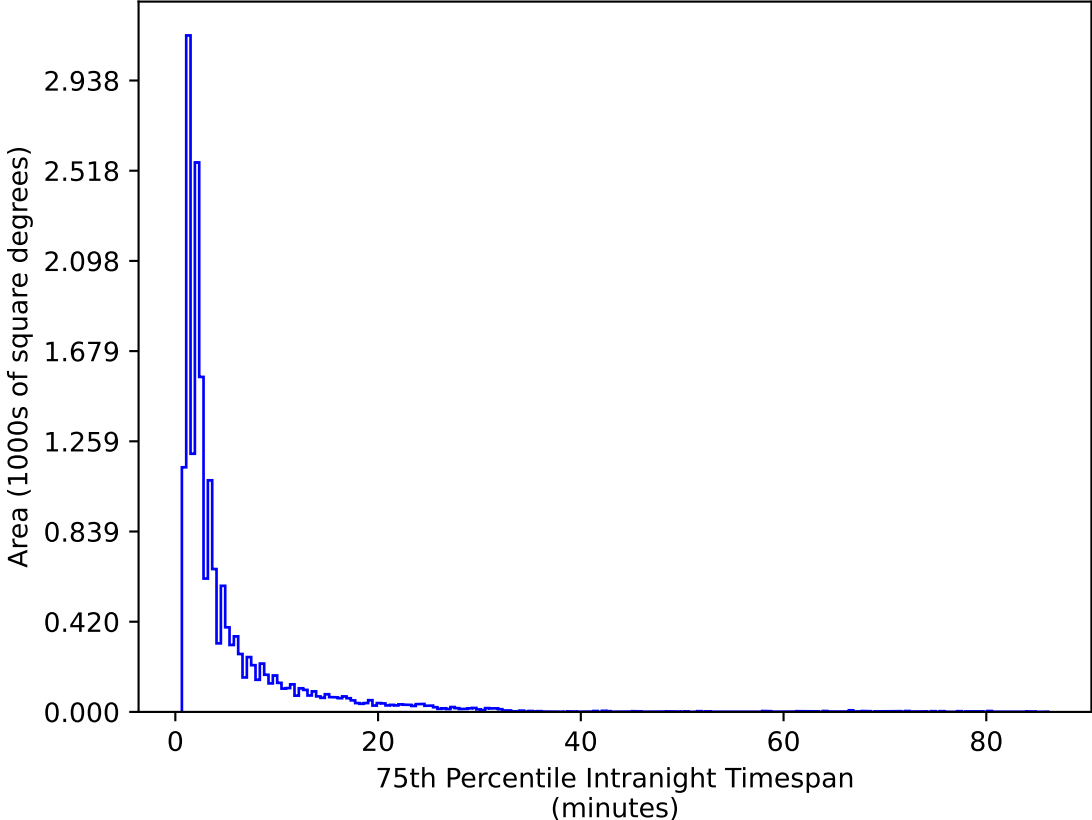
ddf_acor_sf15_lsf30_lsr10_v3.4_10yrs WFD g band: 75th Percentile Intranight Timespan
