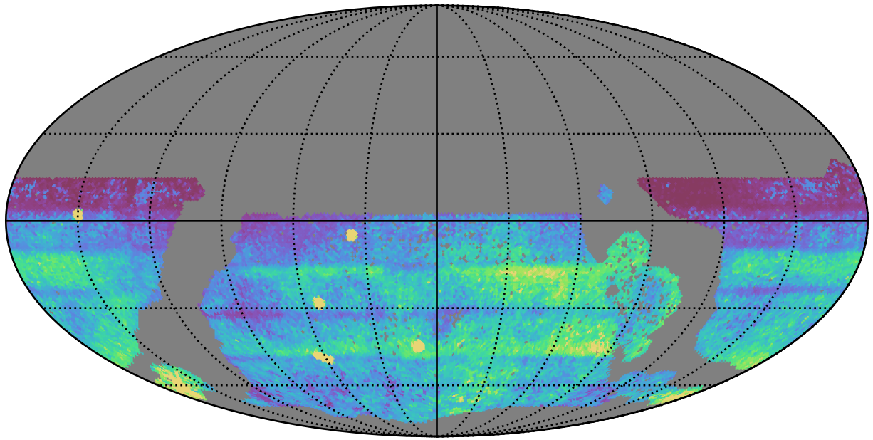
ddf_acor_sf15_lsf30_lsr10_v3.4_10yrs WFD all bands: 75th Percentile Intranight Timespan
