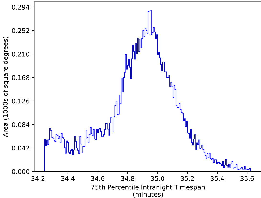
ddf_acor_sf15_lsf30_lsr10_v3.4_10yrs WFD all bands: 75th Percentile Intranight Timespan
