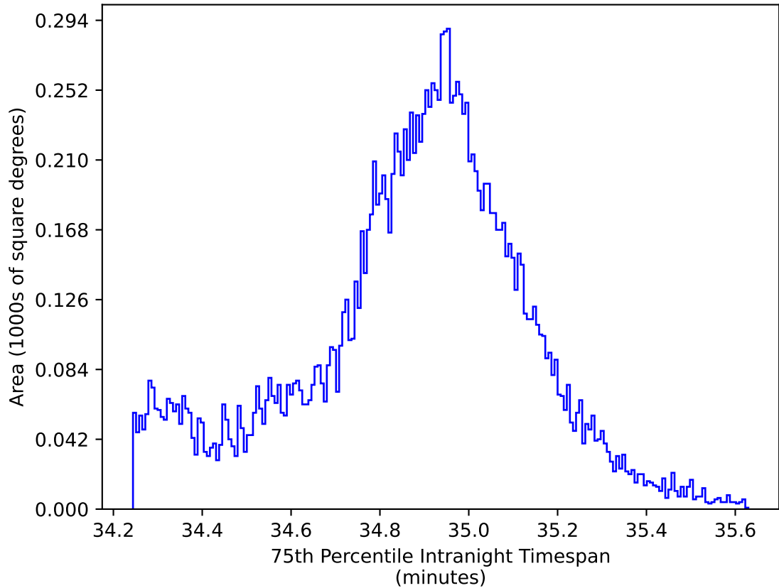
ddf_acor_sf15_lsf30_lsr10_v3.4_10yrs WFD: 75th Percentile Intranight Timespan
