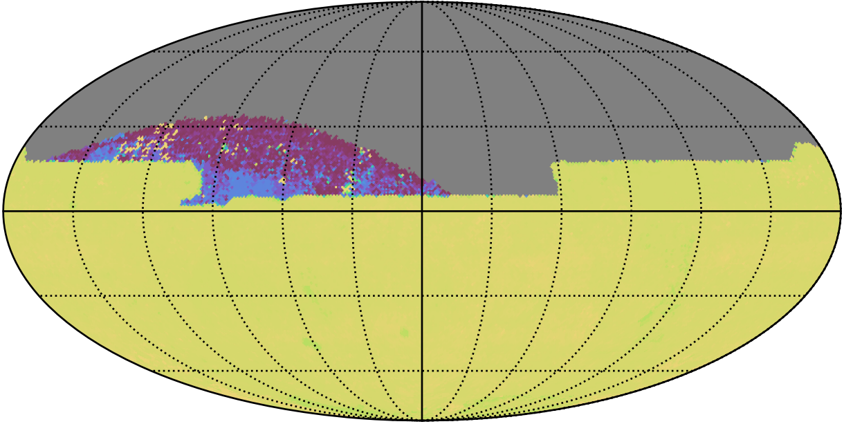
ddf_acor_sf15_lsf30_lsr10_v3.4_10yrs All sky zy bands: 75th Percentile Intranight Timespan
