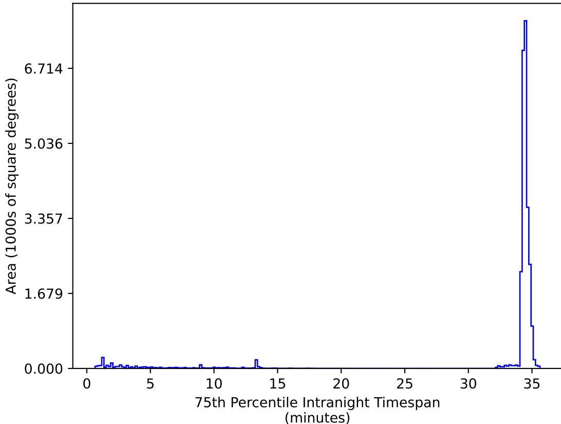
ddf_acor_sf15_lsf30_lsr10_v3.4_10yrs All sky zy bands: 75th Percentile Intranight Timespan
