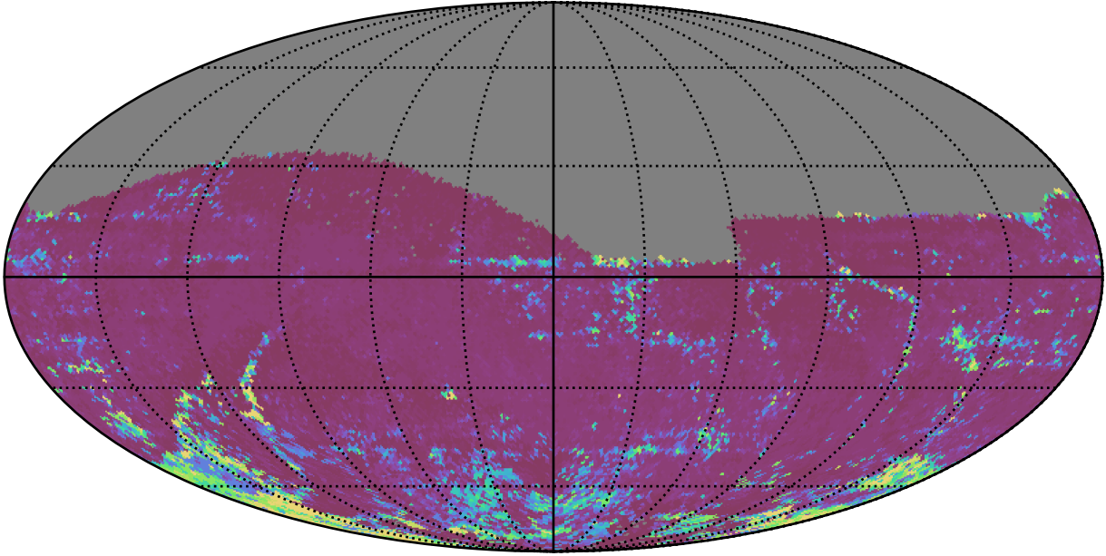
ddf_acor_sf15_lsf30_lsr10_v3.4_10yrs All sky z band: 75th Percentile Intranight Timespan
