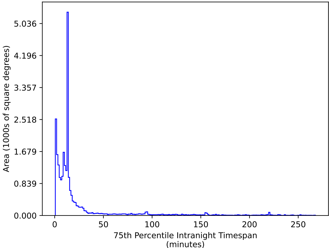
ddf_acor_sf15_lsf30_lsr10_v3.4_10yrs All sky z band: 75th Percentile Intranight Timespan
