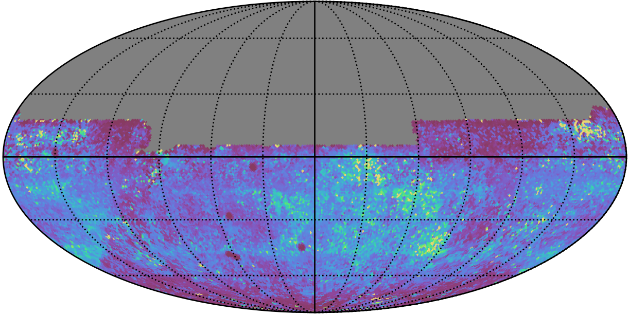
ddf_acor_sf15_lsf30_lsr10_v3.4_10yrs All sky y band: 75th Percentile Intranight Timespan
