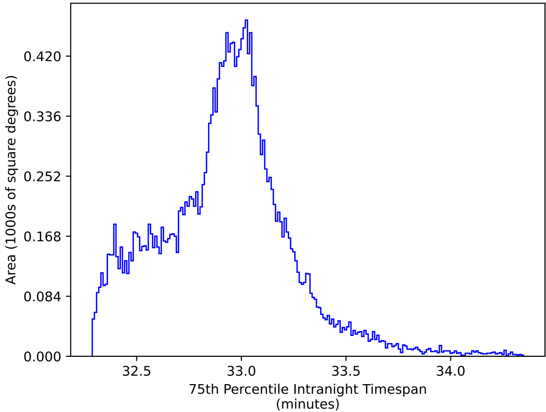
ddf_acor_sf15_lsf30_lsr10_v3.4_10yrs All sky y band: 75th Percentile Intranight Timespan
