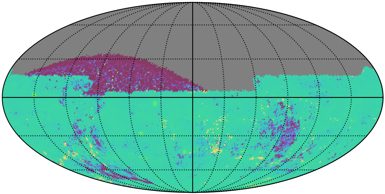
ddf_acor_sf15_lsf30_lsr10_v3.4_10yrs All sky ug bands: 75th Percentile Intranight Timespan
