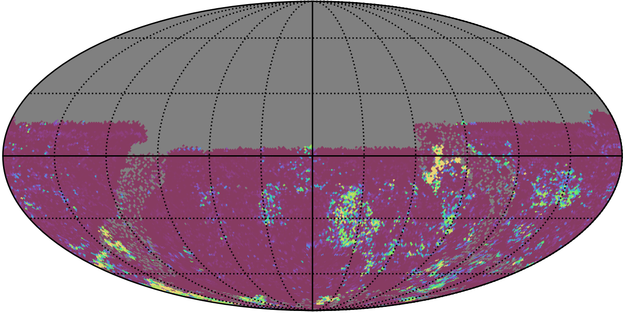
ddf_acor_sf15_lsf30_lsr10_v3.4_10yrs All sky u band: 75th Percentile Intranight Timespan
