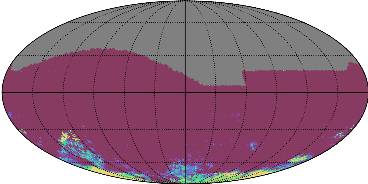
ddf_acor_sf15_lsf30_lsr10_v3.4_10yrs All sky ri bands: 75th Percentile Intranight Timespan
