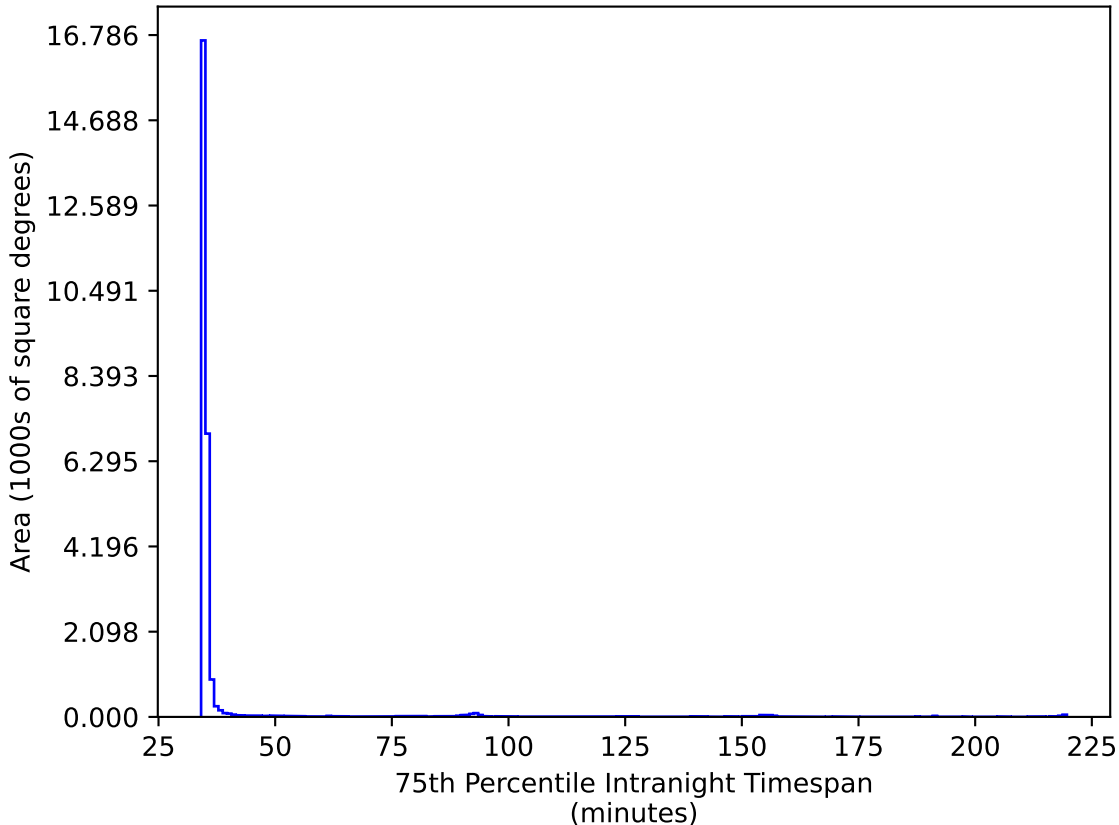
ddf_acor_sf15_lsf30_lsr10_v3.4_10yrs All sky ri bands: 75th Percentile Intranight Timespan
