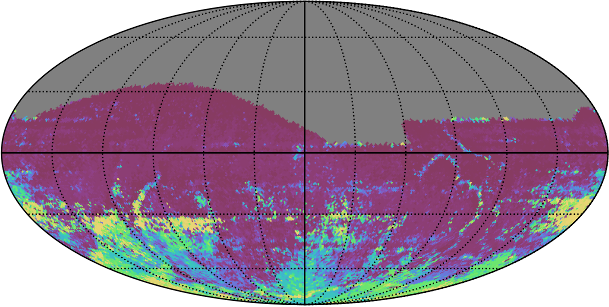
ddf_acor_sf15_lsf30_lsr10_v3.4_10yrs All sky r band: 75th Percentile Intranight Timespan
