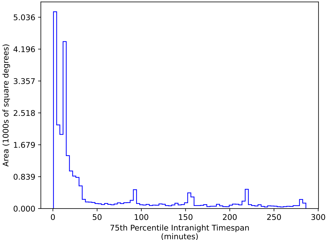
ddf_acor_sf15_lsf30_lsr10_v3.4_10yrs All sky r band: 75th Percentile Intranight Timespan
