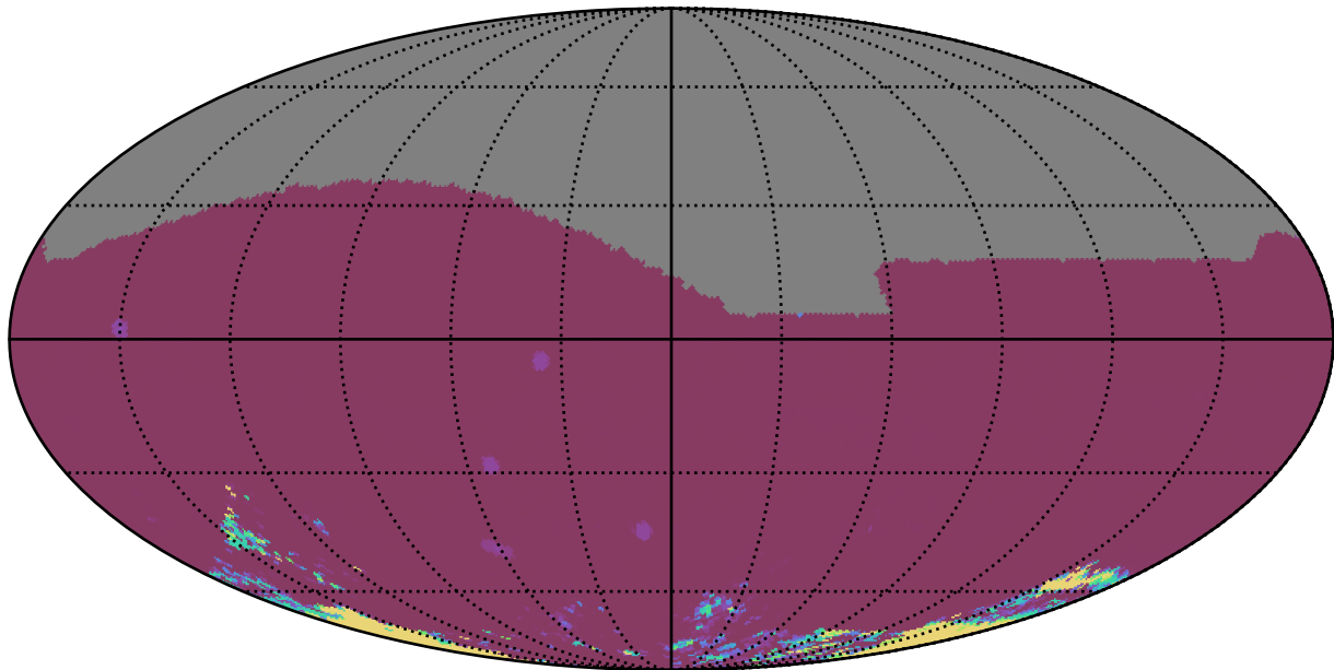
ddf_acor_sf15_lsf30_lsr10_v3.4_10yrs All sky iz bands: 75th Percentile Intranight Timespan
