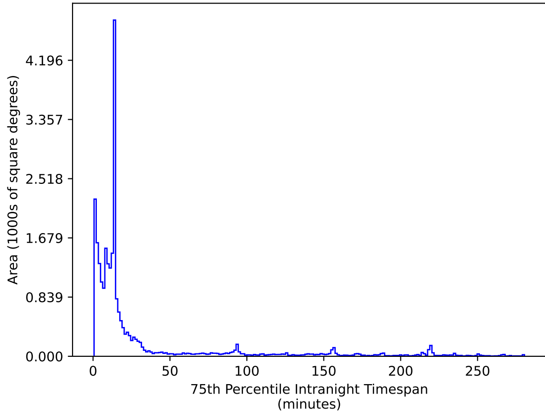
ddf_acor_sf15_lsf30_lsr10_v3.4_10yrs All sky i band: 75th Percentile Intranight Timespan
