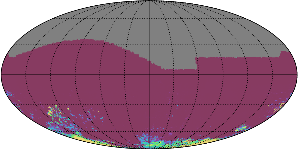
ddf_acor_sf15_lsf30_lsr10_v3.4_10yrs All sky gr bands: 75th Percentile Intranight Timespan
