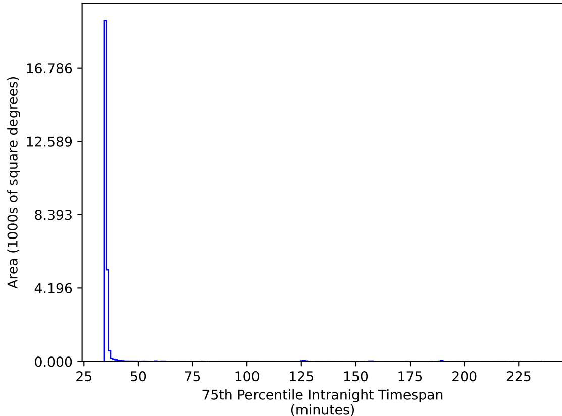
ddf_acor_sf15_lsf30_lsr10_v3.4_10yrs All sky gr bands: 75th Percentile Intranight Timespan
