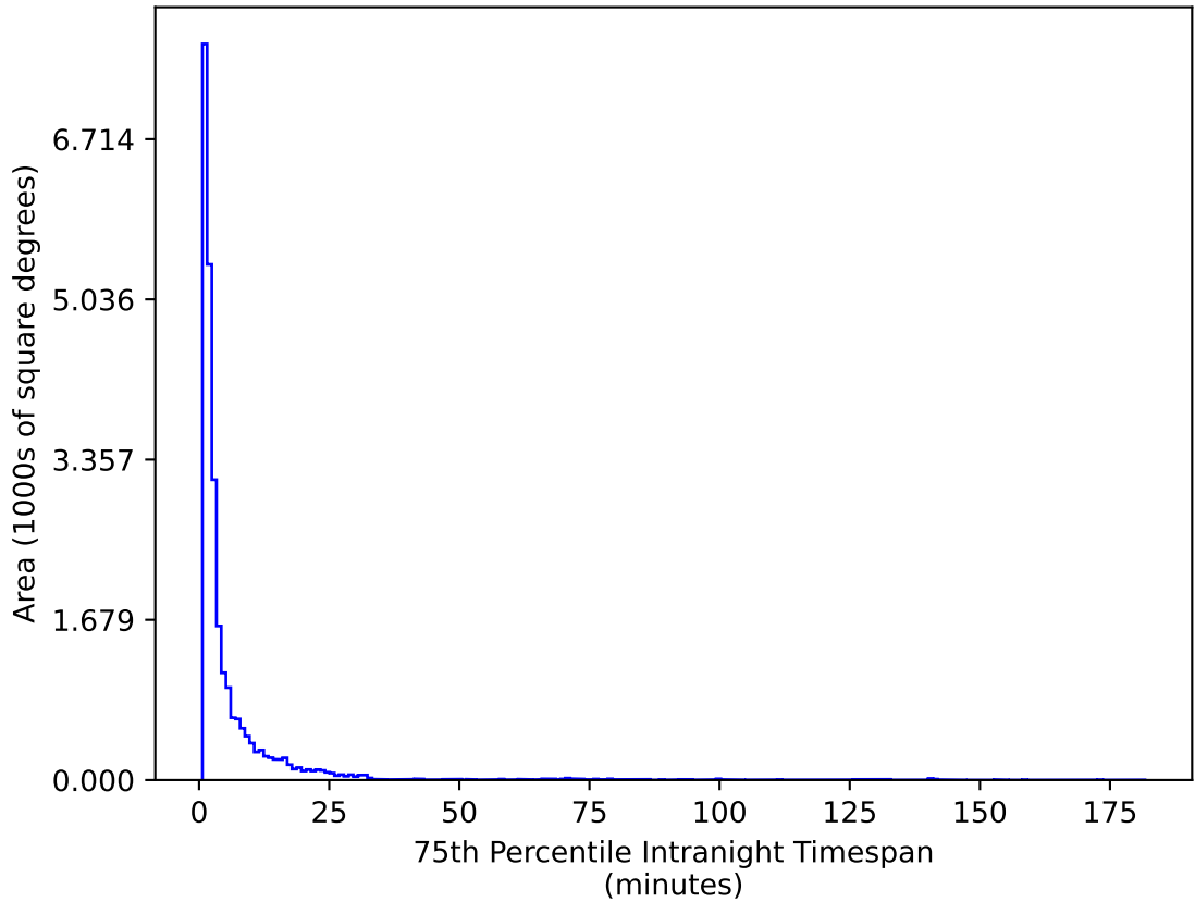
ddf_acor_sf15_lsf30_lsr10_v3.4_10yrs All sky g band: 75th Percentile Intranight Timespan
