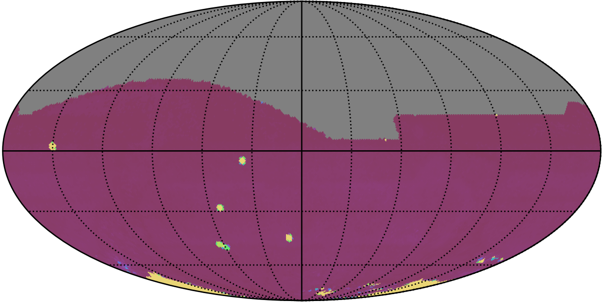
ddf_acor_sf15_lsf30_lsr10_v3.4_10yrs All sky all bands: 75th Percentile Intranight Timespan
