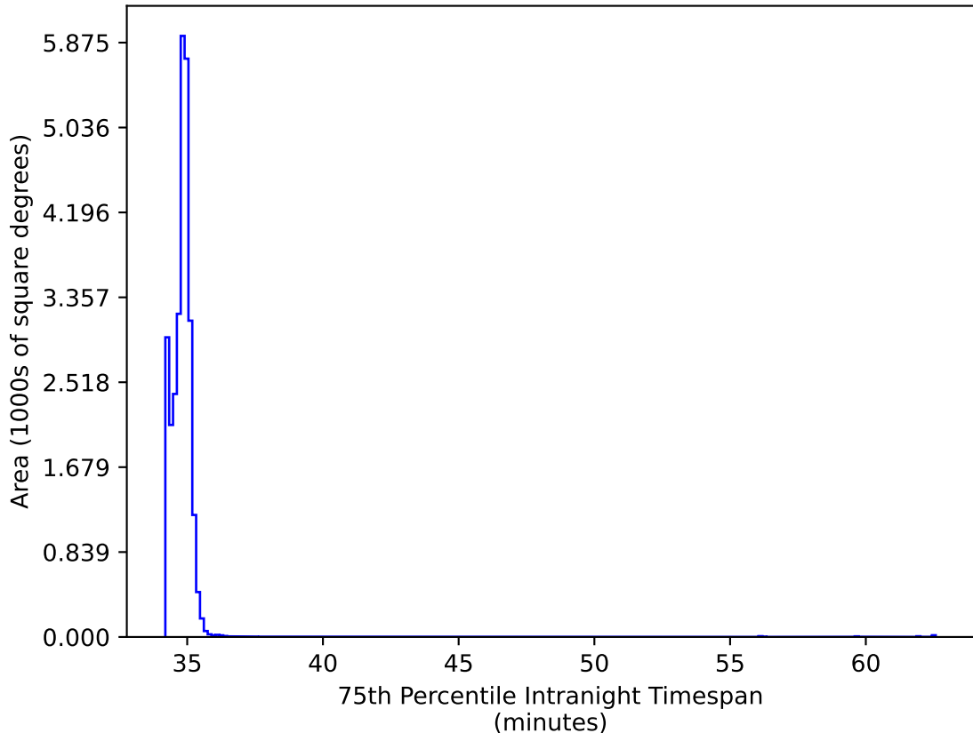
ddf_acor_sf15_lsf30_lsr10_v3.4_10yrs All sky all bands: 75th Percentile Intranight Timespan
