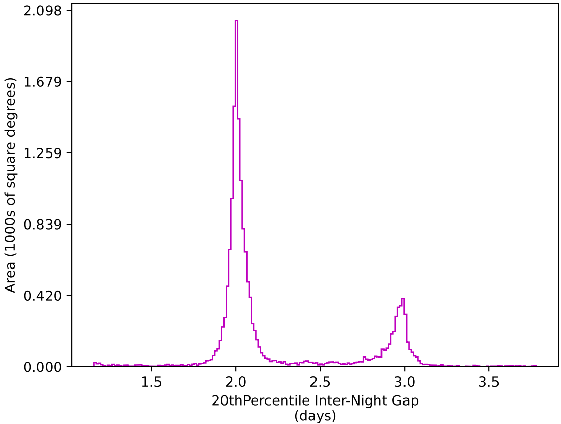
ddf_acor_sf15_lsf30_lsr10_v3.4_10yrs WFD z band: 20thPercentile Inter-Night Gap
