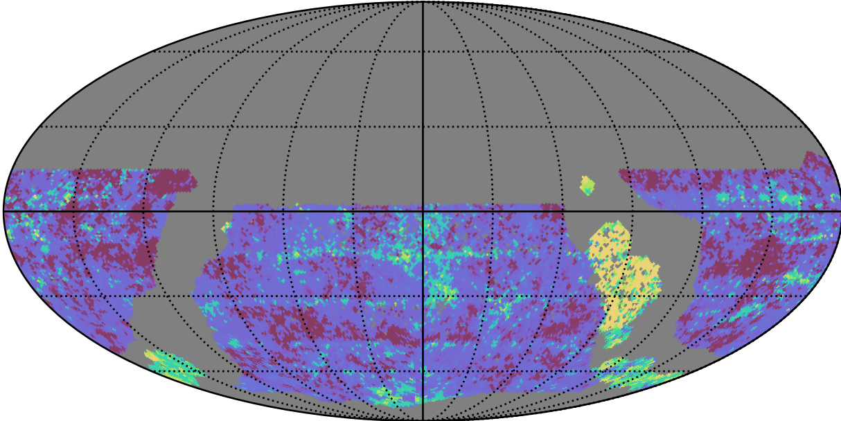
ddf_acor_sf15_lsf30_lsr10_v3.4_10yrs WFD y band: 20thPercentile Inter-Night Gap
