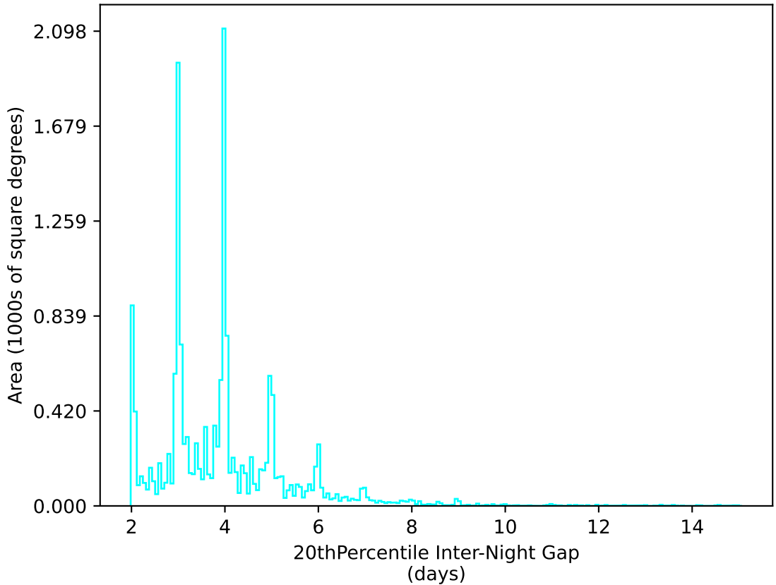
ddf_acor_sf15_lsf30_lsr10_v3.4_10yrs WFD u band: 20thPercentile Inter-Night Gap
