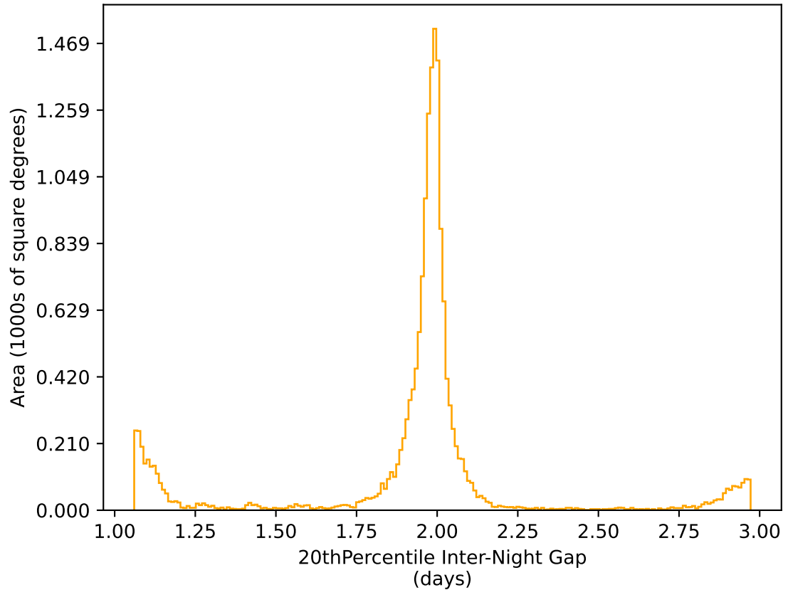
ddf_acor_sf15_lsf30_lsr10_v3.4_10yrs WFD r band: 20thPercentile Inter-Night Gap
