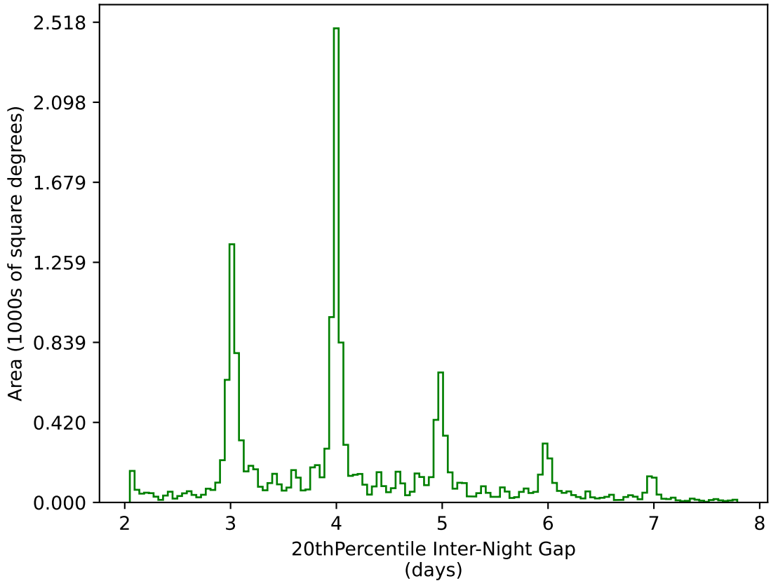
ddf_acor_sf15_lsf30_lsr10_v3.4_10yrs WFD g band: 20thPercentile Inter-Night Gap
