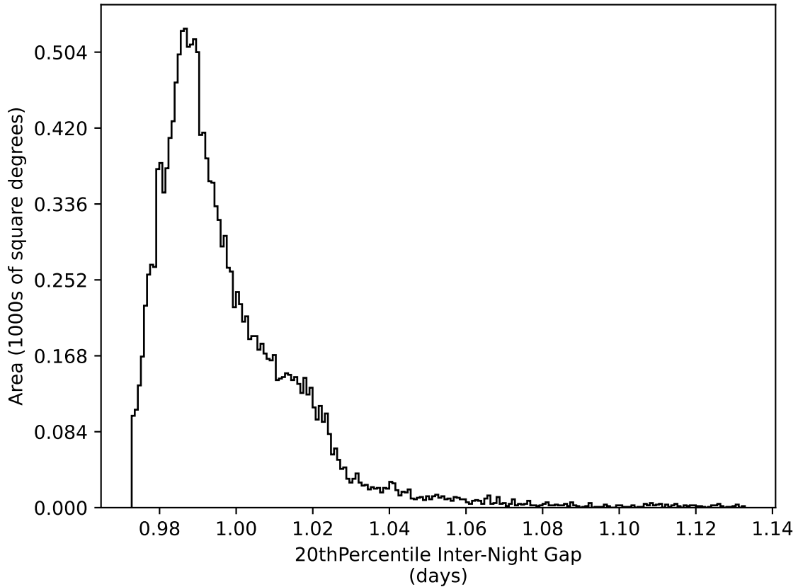
ddf_acor_sf15_lsf30_lsr10_v3.4_10yrs WFD all bands: 20thPercentile Inter-Night Gap
