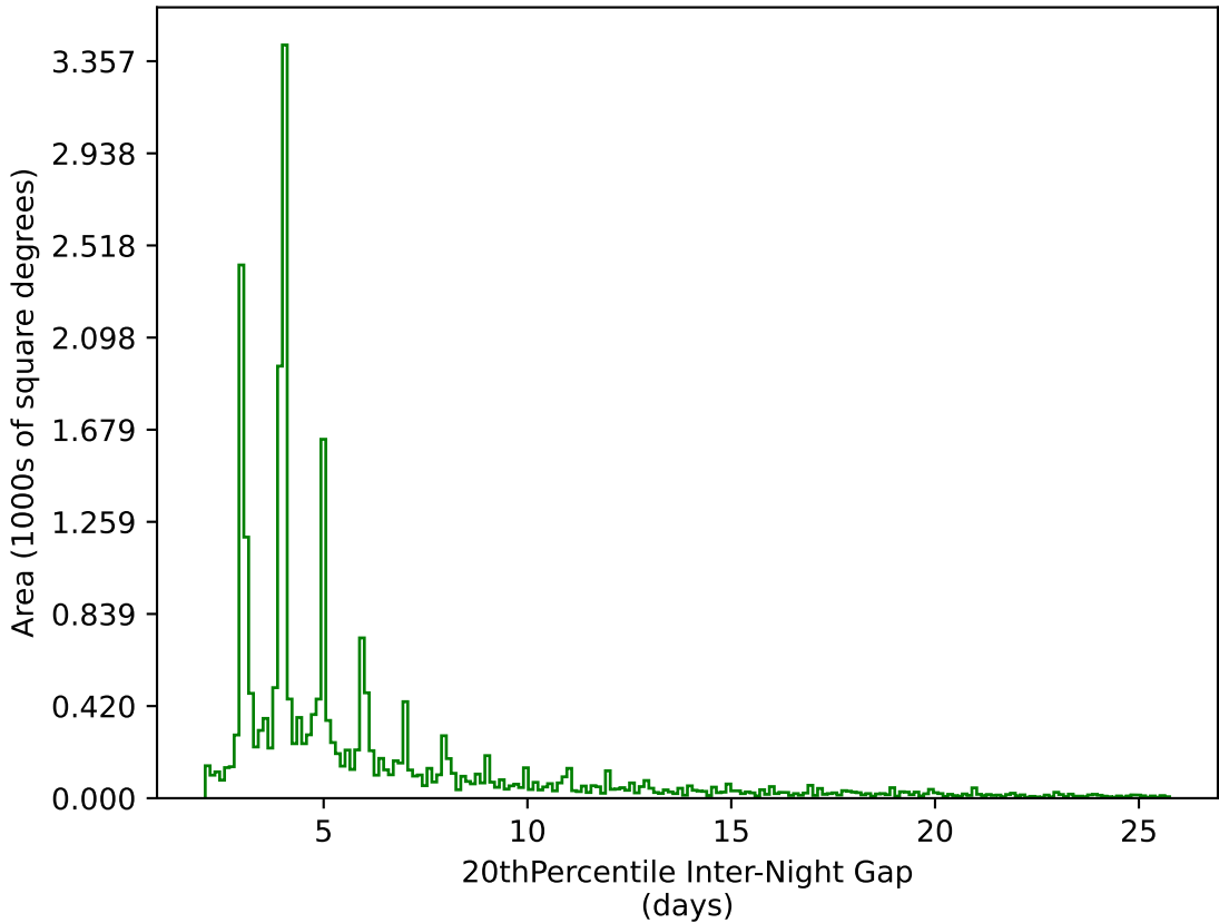
ddf_acor_sf15_lsf30_lsr10_v3.4_10yrs All sky g band: 20thPercentile Inter-Night Gap
