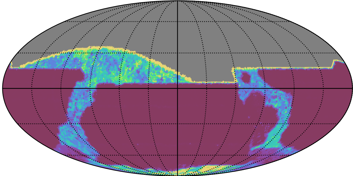
ddf_acor_sf15_lsf30_lsr10_v3.4_10yrs All sky all bands: 20thPercentile Inter-Night Gap
