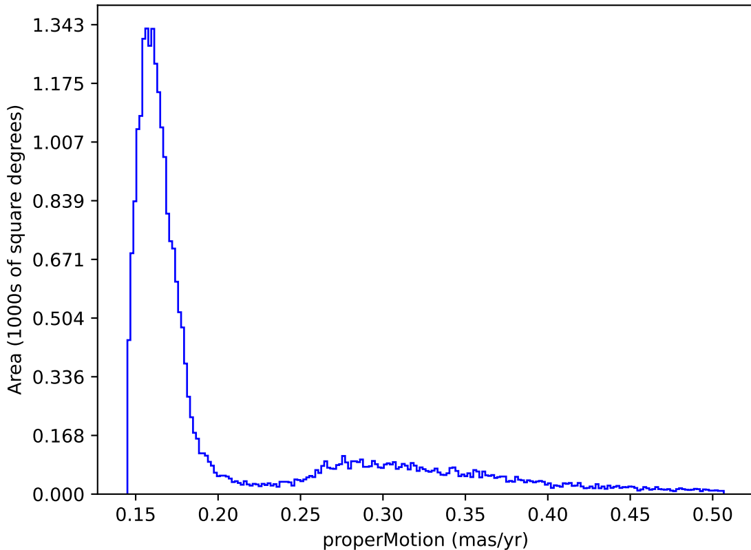
ddf_acor_sf15_ls30_lsr10_v3.4_10yrs : properMotion
