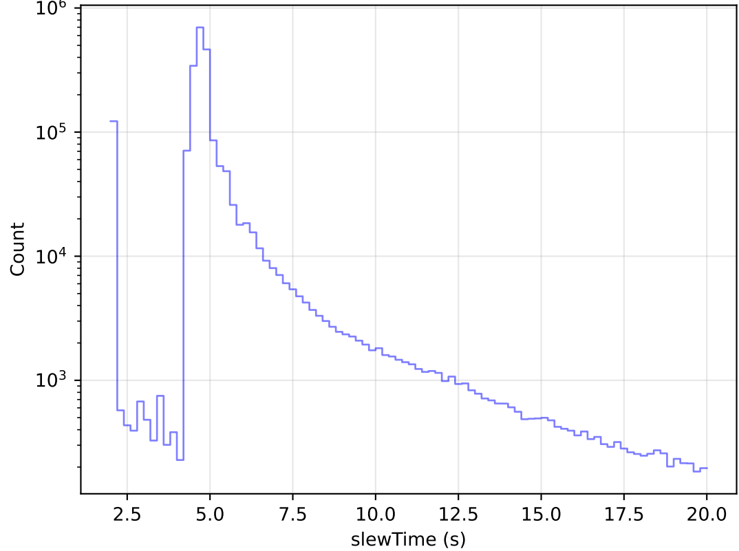
ddf_acor_sf15_Isf30_Isr10_v3.4_10yrs All visits: Zoom Slew Time Histogram
