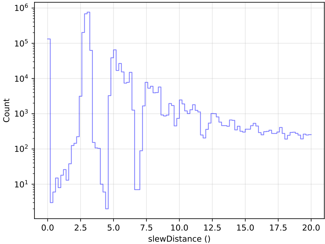
ddf_acor_sf15_lsf30_lsr10_v3.4_10yrs All visits: Zoom Slew Distance Histogram
