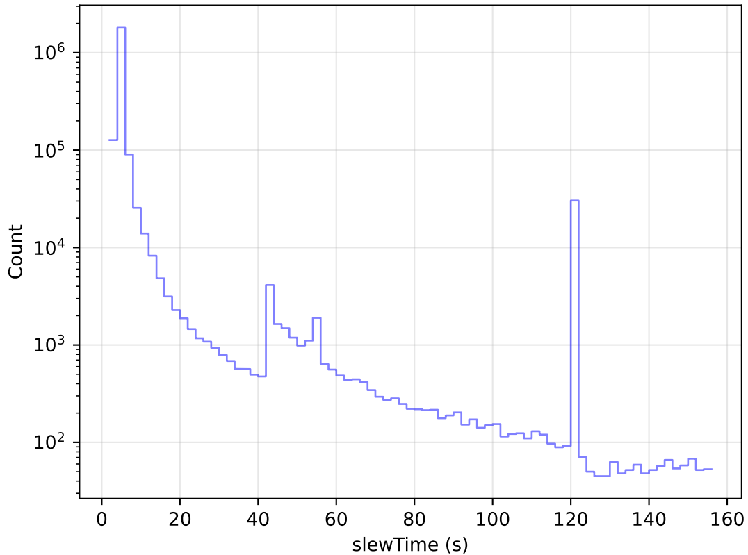
ddf_acor_sf15_lsf30_lsr10_v3.4_10yrs All visits: Slew Time Histogram
