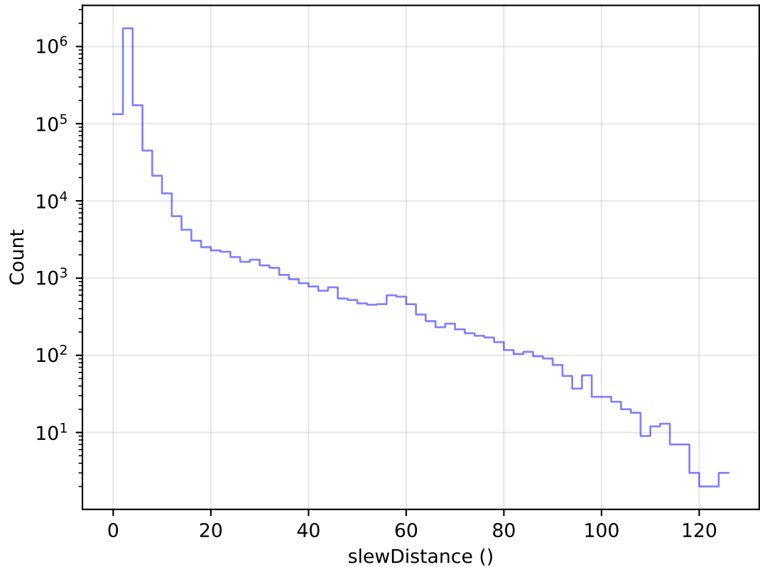
ddf_acor_sf15_lsf30_lsr10_v3.4_10yrs All visits: Slew Distance Histogram
