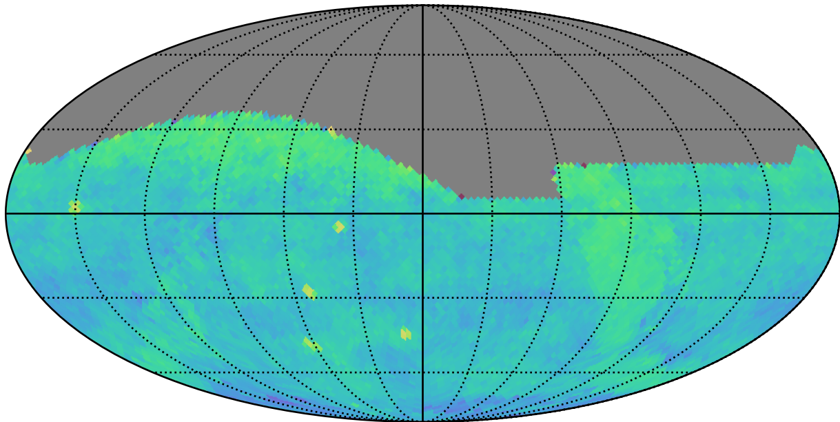
ddf_acor_sf15_lsf30_lsr10_v3.4_10yrs (g or r or i): PairFraction
