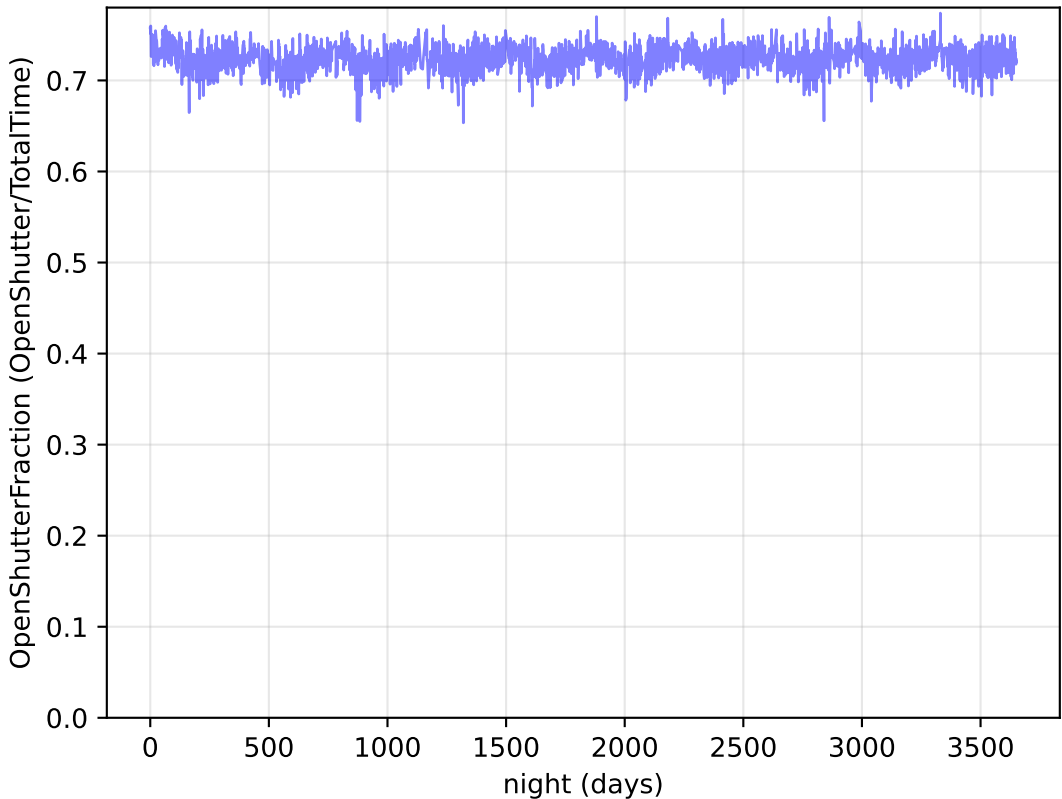
ddf_acor_sf15_lsf30_lsr10_v3.4_10yrs : OpenShutterFraction
