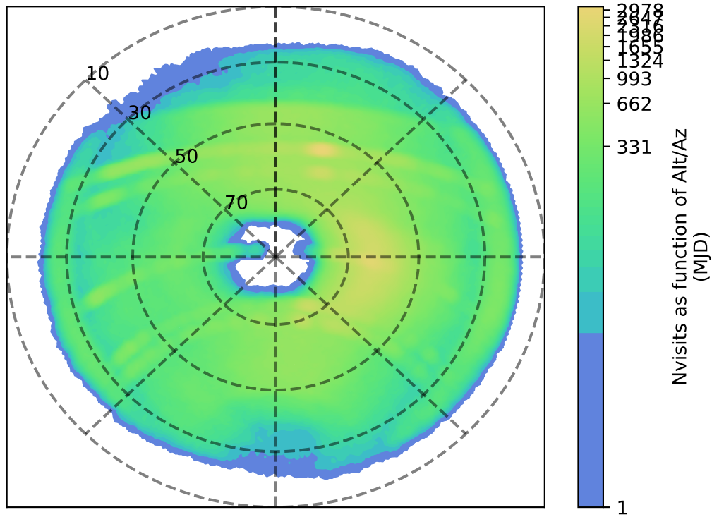
ddf_acor_sf15_ls30_lsr10_v3.4_10yrs z: Nvisits as function of Alt/Az
