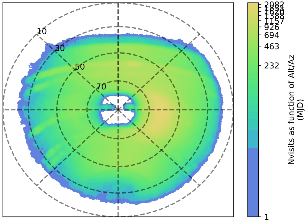
ddf_acor_sf15_lsf30_lsr10_v3.4_10yrs y: Nvisits as function of Alt/Az
