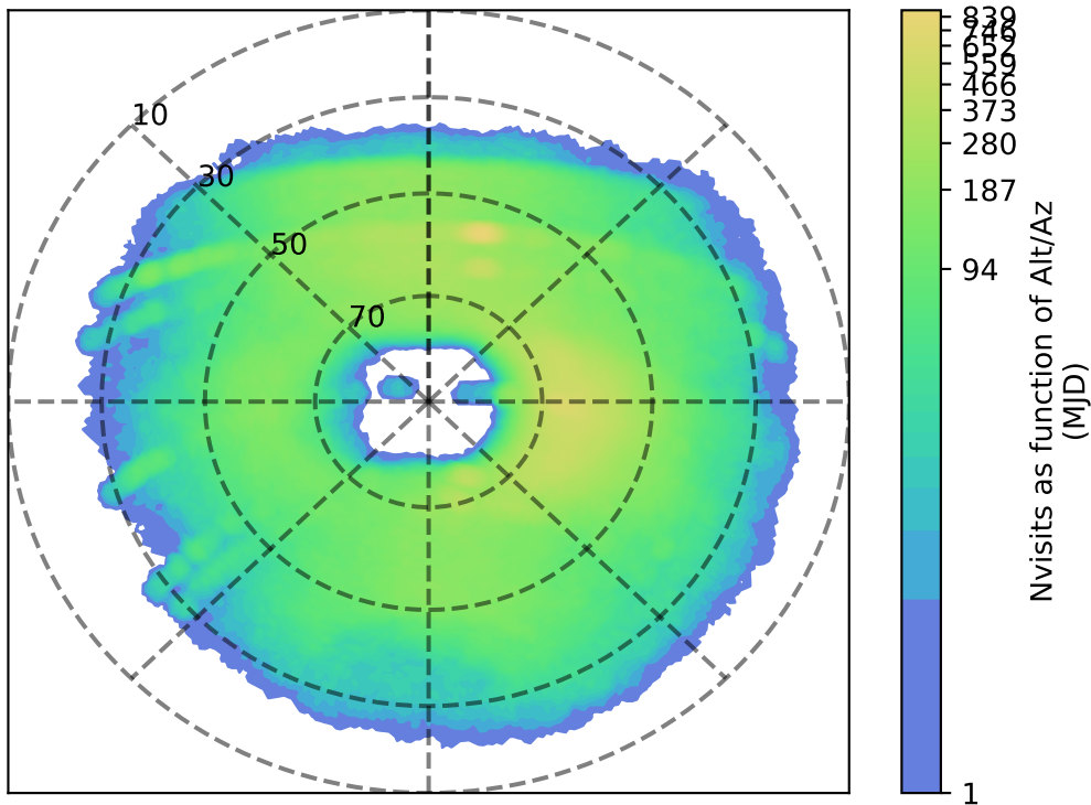
ddf_acor_sf15_ls30_lsr10_v3.4_10yrs u: Nvisits as function of Alt/Az
