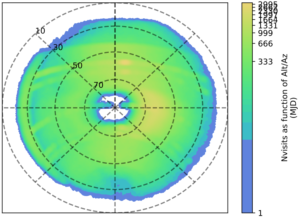
ddf_acor_sf15_ls30_lsr10_v3.4_10yrs r: Nvisits as function of Alt/Az
