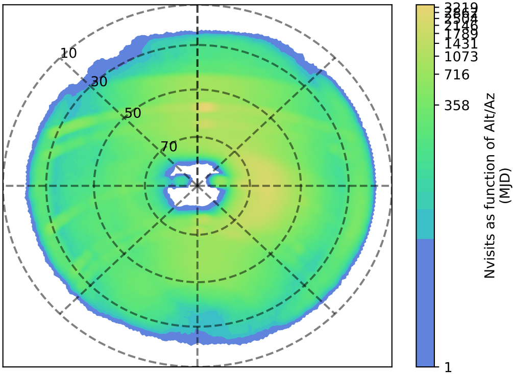
ddf_acor_sf15_ls30_lsr10_v3.4_10yrs i: Nvisits as function of Alt/Az
