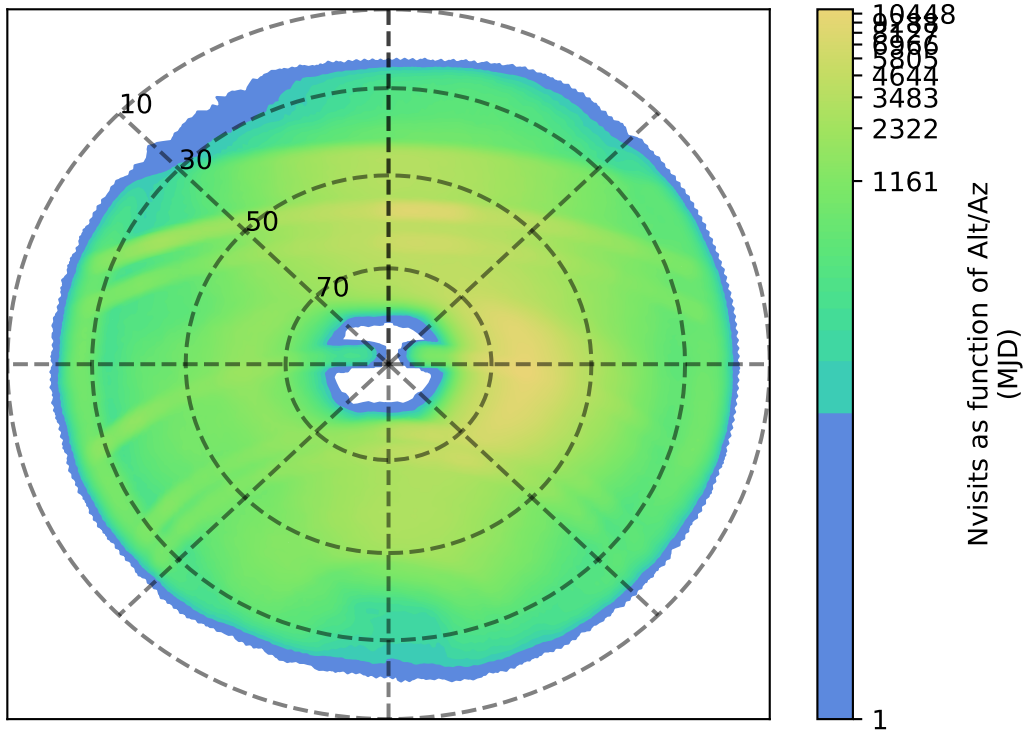
ddf_acor_sf15_lsf30_lsr10_v3.4_10yrs : Nvisits as function of Alt/Az
